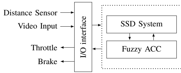
Fig. 1: System architecture for the proposed ADAS
