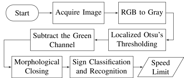
Fig. 4: The speed sign detection and speed limit recognition algorithm
